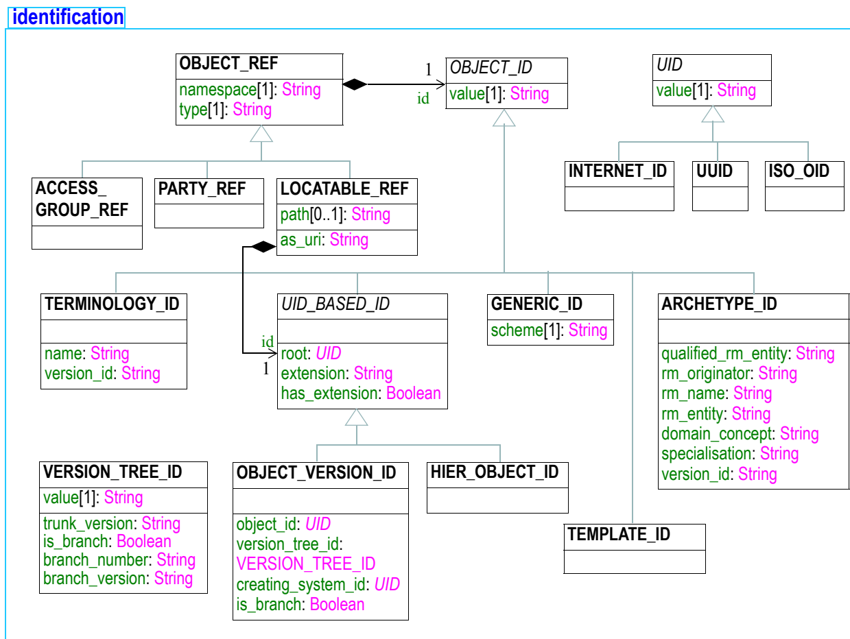
FIGURE 5 rm.support.identification Package
