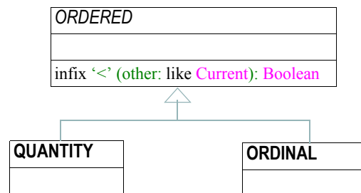
FIGURE 8 pseudo-UML for Anchored Types
