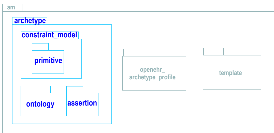
FIGURE 2 openehr.am.archetype Package
