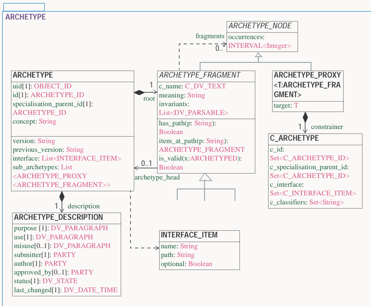
FIGURE 3 AM.COMMON.ARCHETYPE Package
