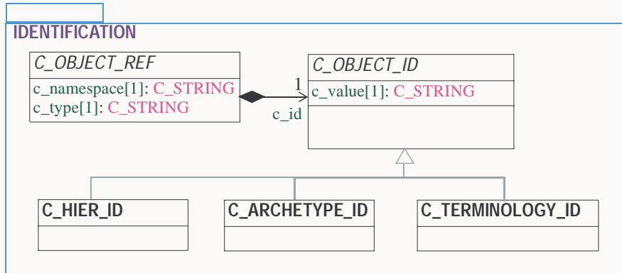
FIGURE 2 AM.COMMON.IDENTIFICATION Package
