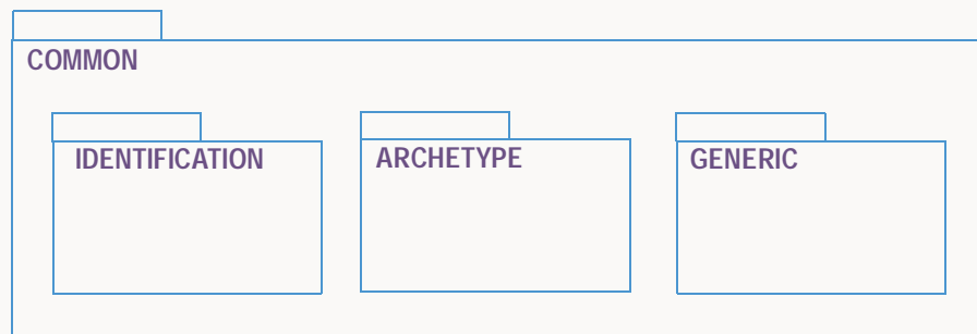
FIGURE 1 AM.COMMON Package
